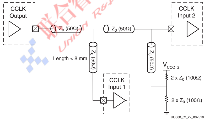
Figure 2-23: Multi-Drop: One CCLK Output, Two CCLK Inputs
