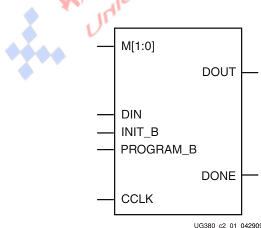
Figure 2-1: Spartan-6 FPGA Serial Configuration Interface
