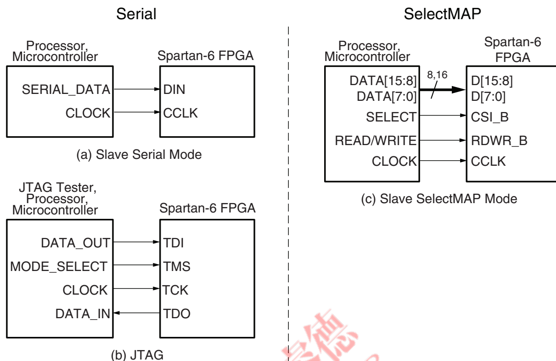
Figure 1-2: Slave Configuration Modes
