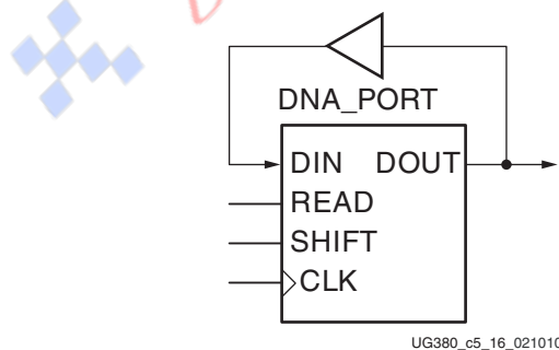
Figure 5-16: Circular Shift
